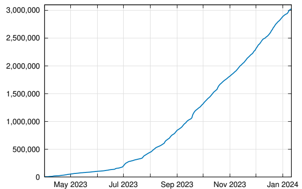
Figure 2: Number of registered users on Bluesky since April 2023.
